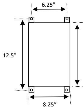
Enclosure Dimensions
