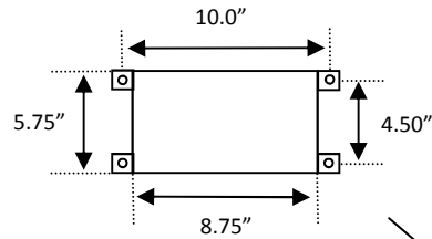
Enclosure Dimensions
